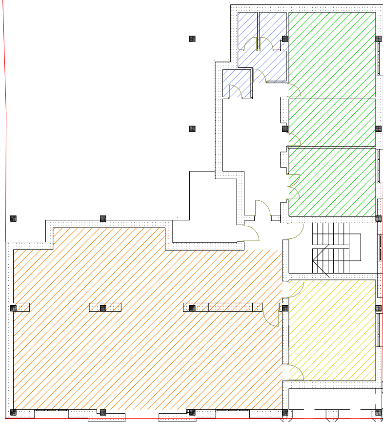
PLAN PARTER PROPUS
