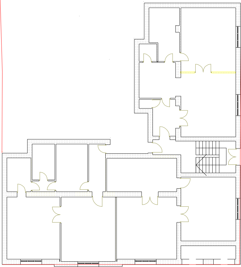
PLAN PARTER EXISTENT
